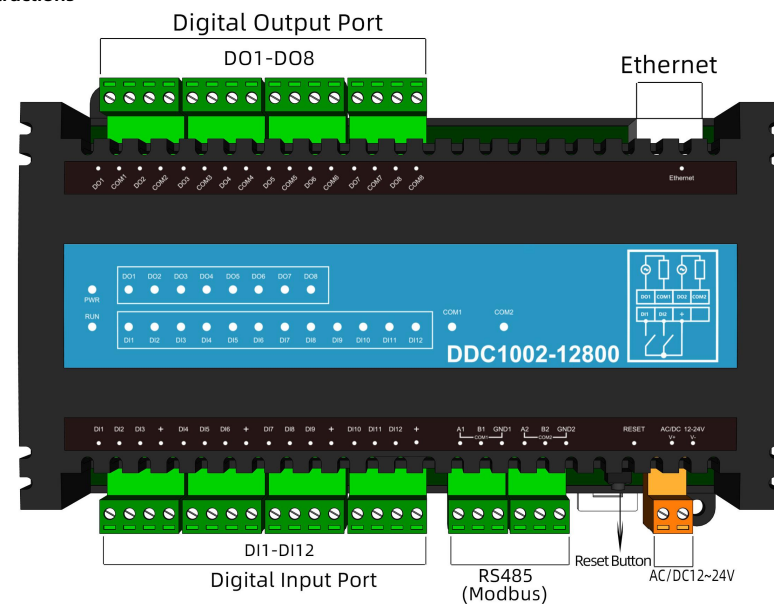
Figure1 Power and Communication Diagram
