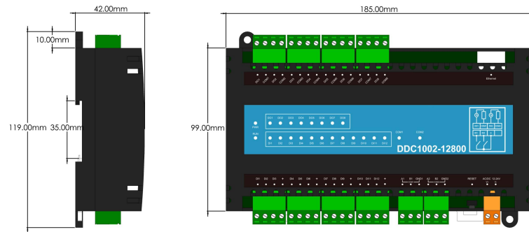
Figure 5 185mm*119mm*42mm(L×W×H) Weight :350g
